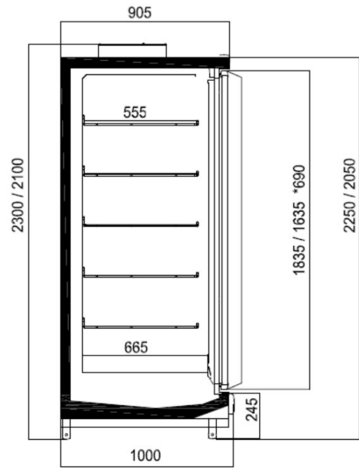
CRYSTAL L
