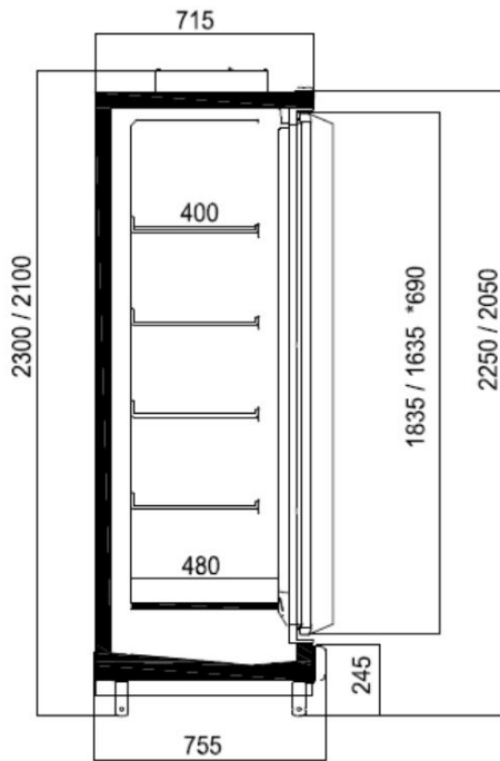
CRYSTAL C
